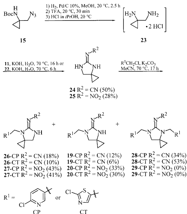
Scheme 4. Preparation of spirocyclopropanated heterocycles 24 , 25 and their N -alkylation with CCMP or CCMT.
