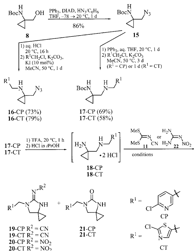
Scheme 3. Preparation of substituted 1-aminocyclopropylmethyl derivatives 16-CP(CT) as well as 18-CP(CT) and cyclizations of the latter with S,S -dimethyl cyanodithioiminocarbonate ( 11 ) and nitroguanidine ( 22 ).
