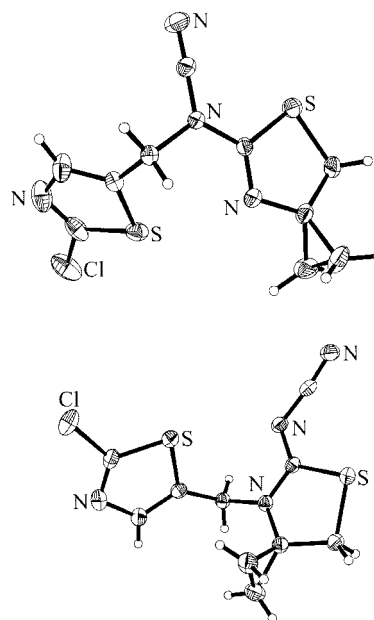
Figure 1. Structures of the chlorothiazole-substituted 6-thia-4-azaspiro[2.4]heptanes 13 -CT and 14 -CT in the crystals. [8]
