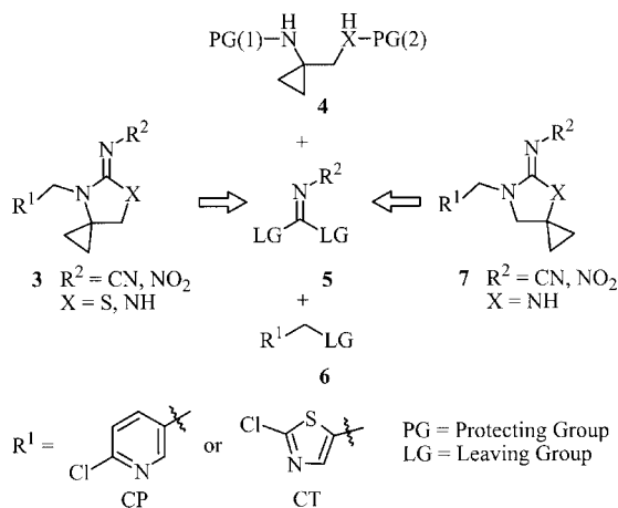
Scheme 1. Retrosynthetic considerations concerning spirocyclopropanated analogues 3 and 7 of Imidacloprid ( 1 ) and Thiacloprid ( 2 ).
