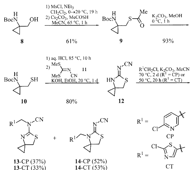
Scheme 2. Synthesis of spirocyclopropanated analogues 14 -CP and 14 -CT of Thiacloprid ( 2 ).
