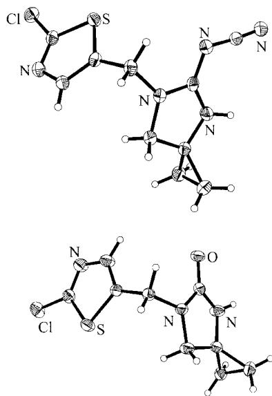
Figure 2. Structures of the spirocyclopropanated analogue 19-CT of Imidacloprid ( 1 ) and the spirocyclic urea derivative 21-CT in the crystals. [8]
